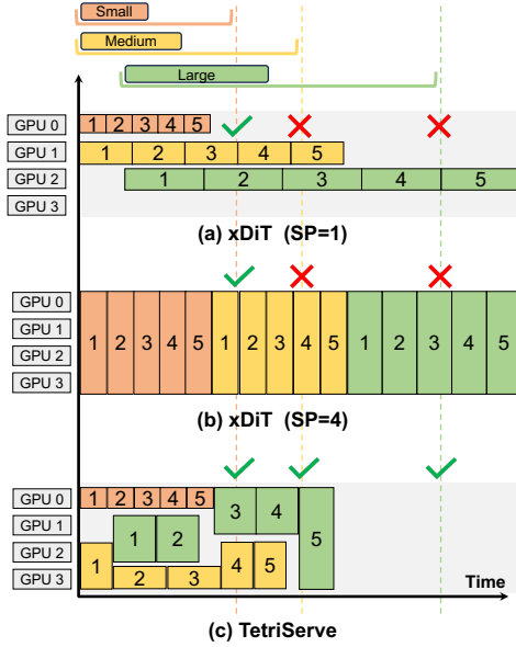
Figure 1. Three DiT serving requests—each with 5 denoising steps—arrive over time with different SLOs and output resolutions. DiT serving solutions using static parallelism cannot adapt and fail to meet multiple SLOs. TetriServe meets more SLOs via SLO-aware scheduling and packing.
